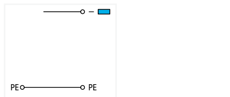
Actuator supply terminal block; with ground connection; power supply from control panel side; with end plate Terminal block width: 6 mm / 0.236 inch
