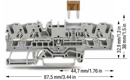
4-conductor fuse terminal block; for mini-automotive blade-style fuse; with test point Electrical ratings are given by the fuse. Blade-style fuses: Observe touch-proof protection for 42 V and higher voltages!
