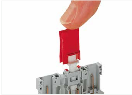
Installing a disconnect lock on the terminal block's disconnect tab (picture shows a 2-pin disconnect carrier terminal block, 769 Series).
