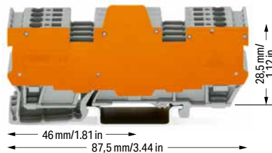
1-conductor/1-conductor terminal block for pluggable modules; with two jumper positions; with orange separator plate; gray
