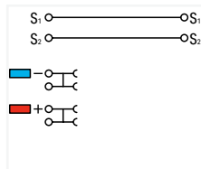
3-conductor sensor terminal block
