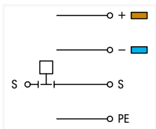
Sensor terminal block; with ground connection; for component plugs
