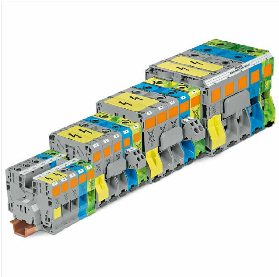
Group marker carriers for WAGO Rail-Mount Terminal Blocks TOPJOB® S – can be snapped into jumper slots.
