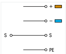
Sensor terminal block; with ground connection
