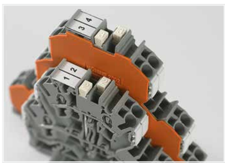
Created for double- and triple-deck terminal blocks TOPJOB® S, the vertical jumpers can common two or three levels. Clearly marked numerals ("2" and "3") distinguish the double-deck (2002-492) and triple-deck vertical jumpers (2002-493), even when inserted.
