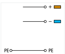
Sensor supply terminal block; with ground connection; power supply from sensor side
