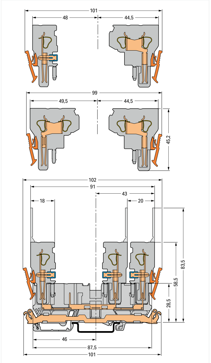
Carrier terminal block; with shield contact
