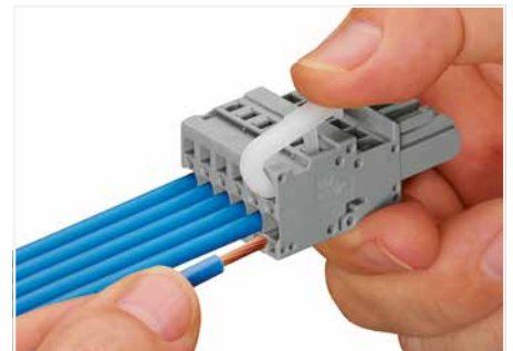
Operating lever Conductor termination – side-entry wiring (example shows a female plug)
