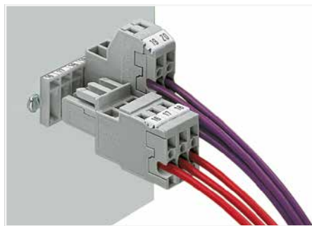
Male header; with feedthrough flanges 1-conductor female plug 2-conductor female plug
