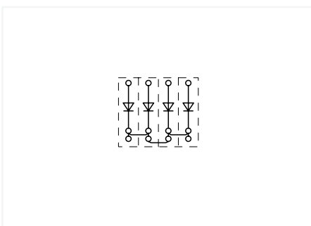
Polarized diode gates with a common cathode can be created using the following terminal blocks: 2004-1311/1000-400 or 2004-1311/1000-401
