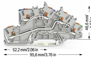
Multilevel installation terminal block; with push-button; gray
