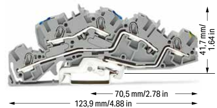
Multilevel installation terminal block; gray
