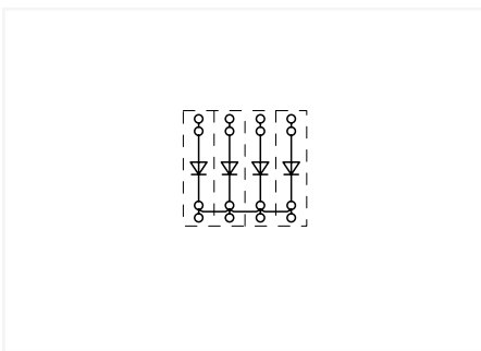
Polarized diode gates with a common cathode can be created using the following terminal blocks: 2004-1411/1000-400 or 2004-1411/1000-401
