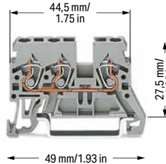
3-conductor through terminal block; for DIN-35 rail
