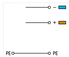
Sensor supply terminal block; with ground connection; power supply from control panel side; with end plate Terminal block width: 6 mm / 0.236 inch
