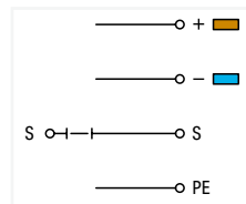
Sensor disconnect terminal block; with ground connection; for signal interruption
