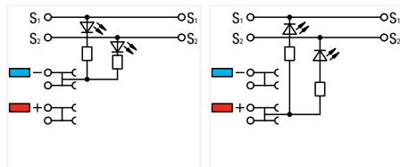
3-conductor sensor terminal block; yellow LED; for PNP (high-side) switching sensors
